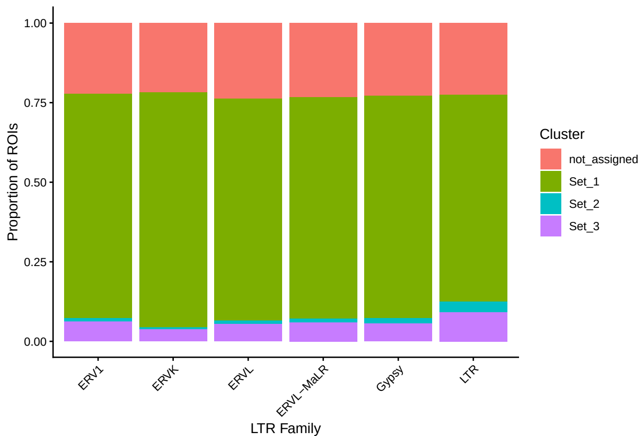
Proportion of ROI summits across each LTR family
